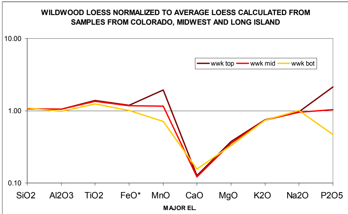
Fig 5 Wildwood loess compared with the average of loess calculated from samples collected in Colorado, Midwest and Long island. There is no large Fe enrichment but there is Ca depletion is still present
