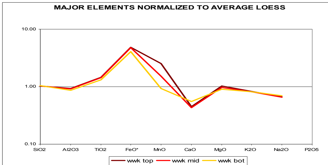
Fig. 4. Wildwood State Park loess normalized to average loess from Schentger, 1992. shows large enrichment in Fe and depletion in Ca. Ca is probably leached from the soil because Long Island soil is acidic.
