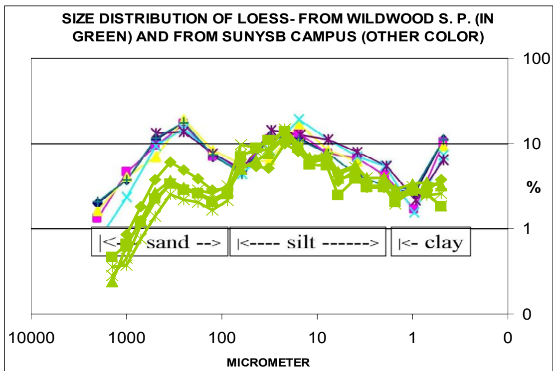
Fig. 3. Grain size distribution of loess from Wildwood State Park is shown as green lines and distribution from SUNYSB campus shown as blue, yellow, pink and light blue lines. Wildwood State Park loess is missing the clay peak and much less sand.
