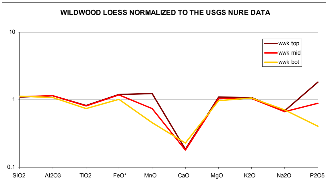
Fig 6. Long Island loess normalized to the likely chemistry of the source shows the Ca depletion and a change in Mn concentration with depth which may be a consequence of soil processes. P is enriched in comparison with the potential source.
