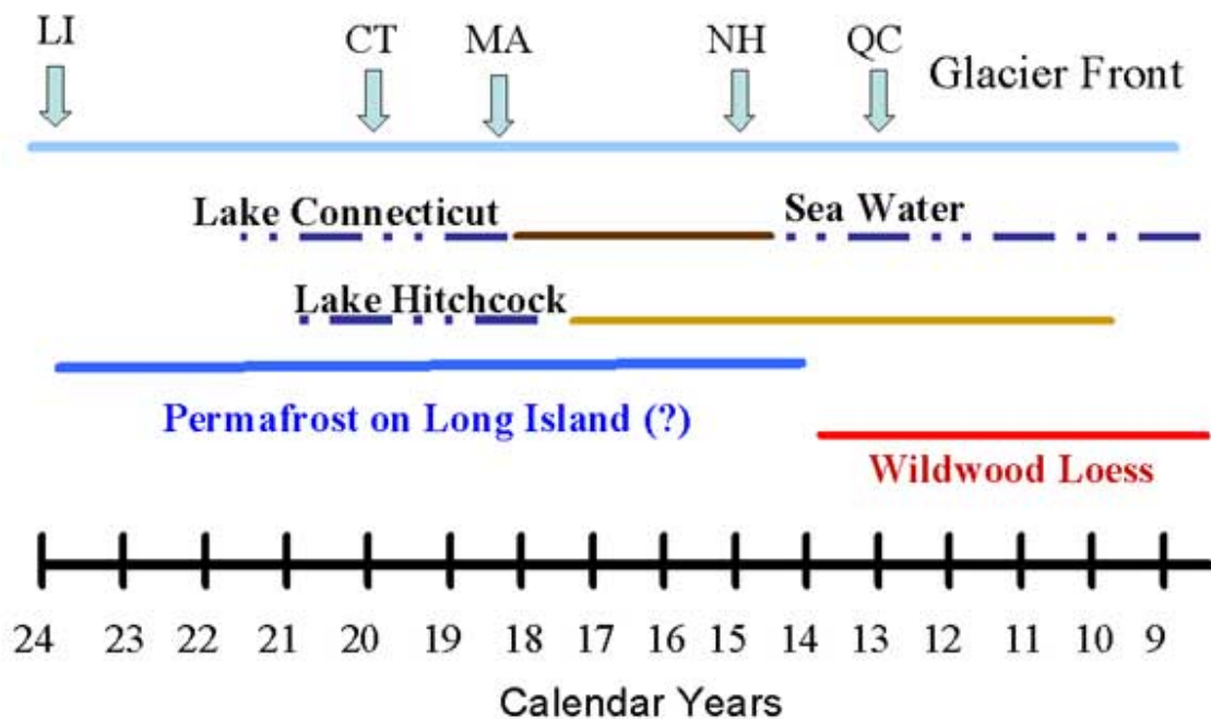
Fig.7. Calendar ages in Ka BP, horizontal lines represent approximate time span of events. Radiocarbon ages have been converted to calendar ages (Stuiver, et al, 1998) The position of the front of the continental glacier after retreating from Long Island (LI) when it first reached Connecticut (CT), Massachusetts (MA), New Hampshire (NH) and Quebec (QC). Light and dark brown lines represent time after Glacial Lake Hitchcock and Glacial Lake Connecticut drained and their lake bottoms were dry with glacial melt water streams crossing the lake bottoms. Broken blue line represents the time when fresh water or sea water was occupying the lake basins. The dark blue line is the time when Long Island may have had permafrost. The Red line shows period of deposition of loess in Wildwood State Park kettle hole as measured with OSL and radiocarbon ages.
